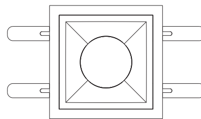
Cutout: 125x125mm Ceiling Spec: 8-15mm Thick
