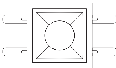
Cutout: 105x105mm Ceiling Spec: 8-15mm Thick
