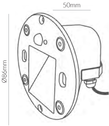
Cutout: Ø68mm
