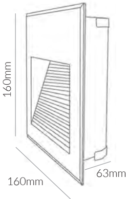
Cutout: 150x60mm
